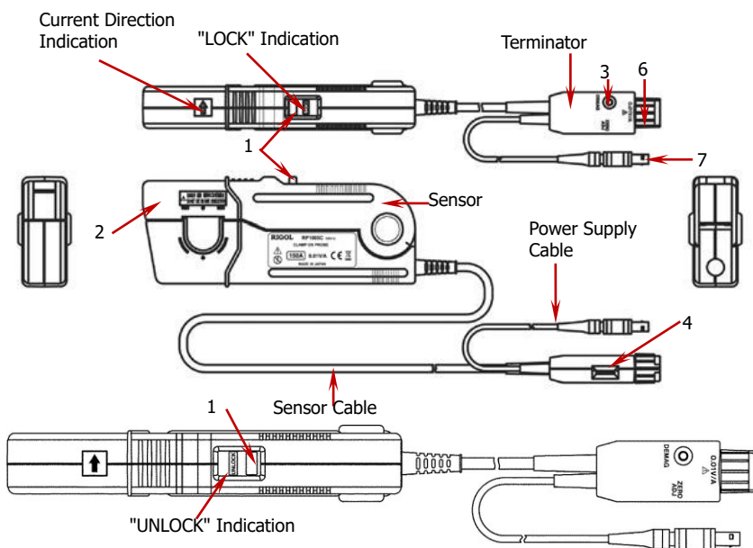
Figure 2 RP1005C/RP1006C Parts
